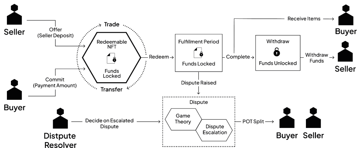
Fig. 2 - How Boson Protocol works
